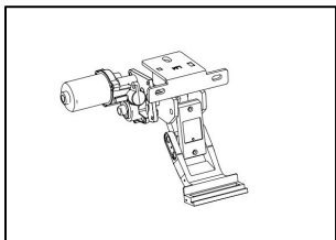
Motor bracket
